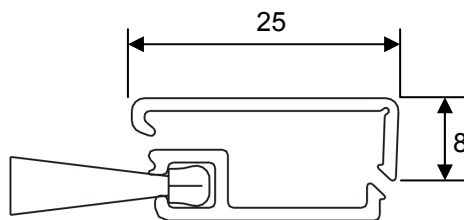
TYPE B JAMB AND LINTEL
