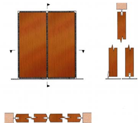
External double timber door
