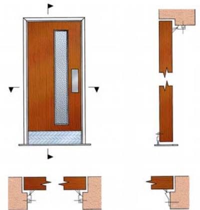
Internal single timber door
